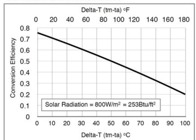
Collector Performance Curve
